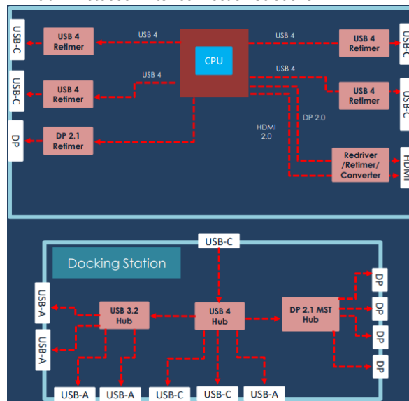
Exhibit 4: Notebook Inter-connection solutions
